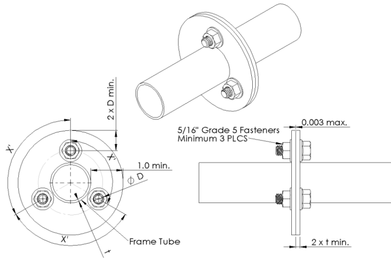
Figure B-28: Roll Cage, Required Joint for Removable Members
