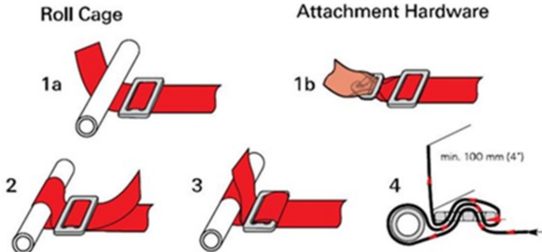
Figure B-34: Driver Harness, Shoulder Harness Lateral Restraint
