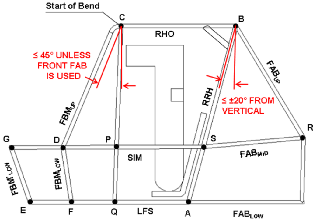
Figure B-22: Roll Cage, FBM
