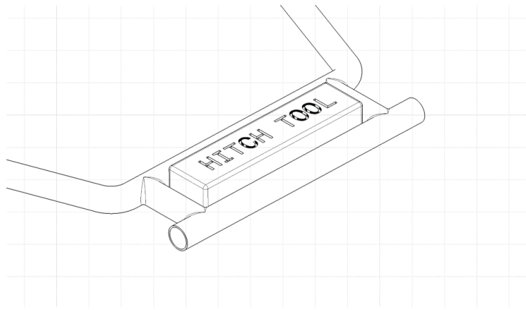
Figure B-59: Tow Point, Inspection Tool Fitment
